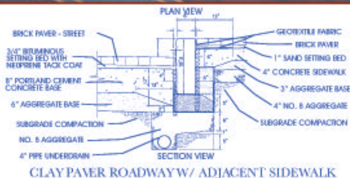
Detail of roadway/curb/sidewalk.
